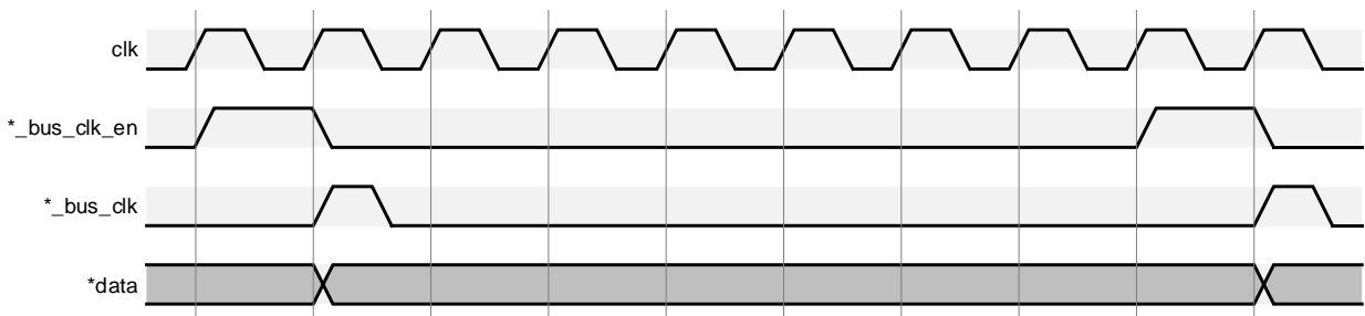
Figure 14-9 1:8 System Bus-to-Core Clock Ratio
